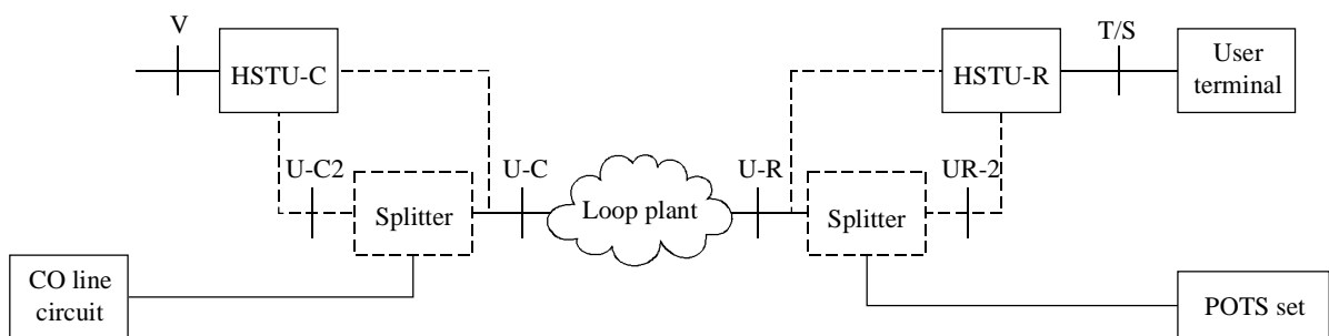
FIGURE 1/G.994.1 System reference model
